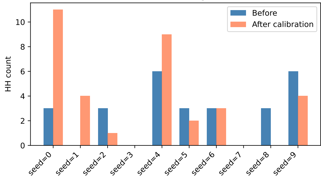
HH count: before vs after — ('german', 'isotonic')
