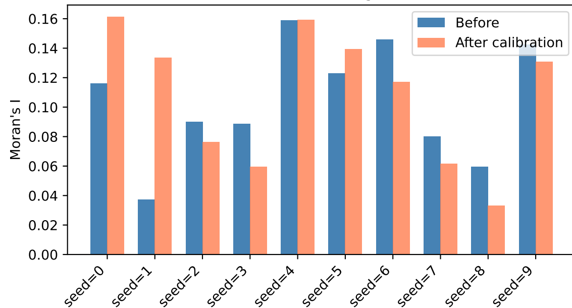
Moran's I: before vs after — ('german', 'isotonic')
